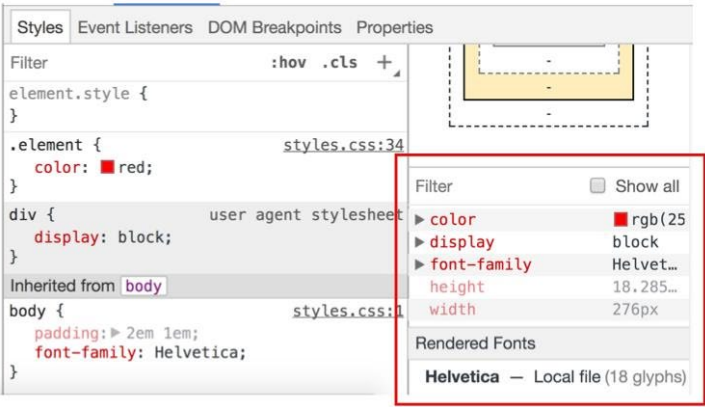
Chrome Devtools (wide width)
